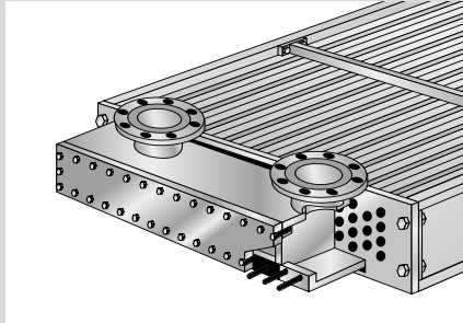
Cover plate header with stud bolts
