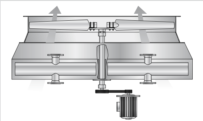
Belt drive for induced draft configuration
