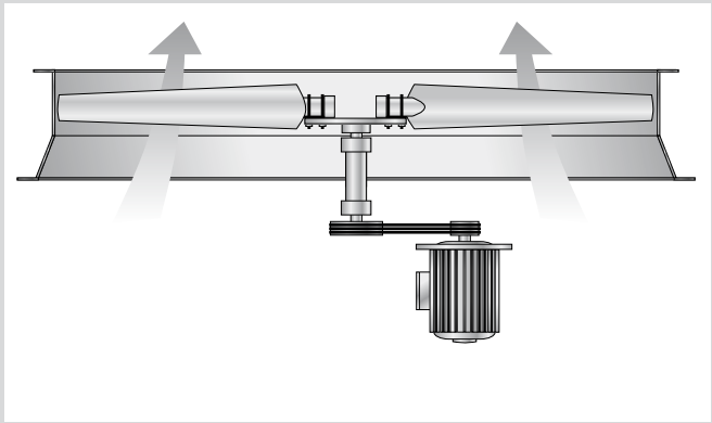
Belt drive for forced draft configuration
