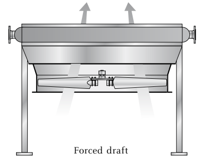
Forced draft
