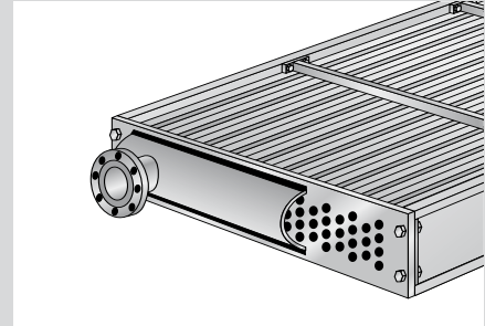
Welded header (D type)
