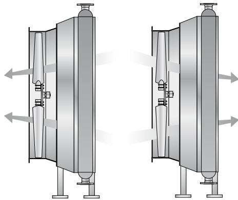
Induced draft
